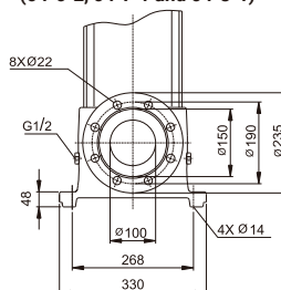
Flange (DIN) PN 25-40 / DN100 (64-6-2, 64-7-1 and 64-8-1)
