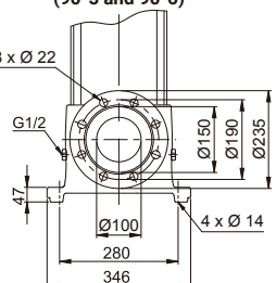
Flange (DIN) PN 25-40 / DN100 (90-5 and 90-6)
